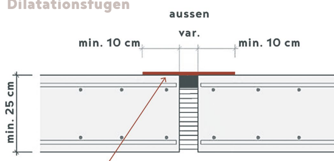
Dilatationsfugen
